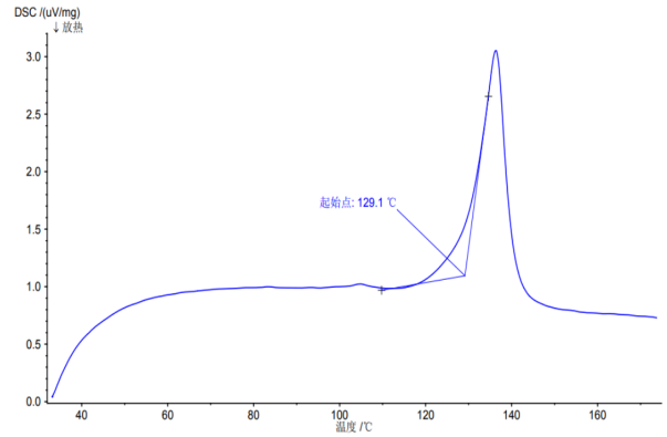
易溶合金熔点测试图 Diagram of melting point test for Fusible Alloy
